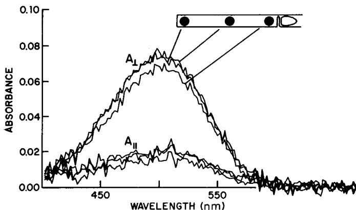
FIGURE 4 Absorbance measurements for light linearly polarized parallel ( A_{||} ) and perpendicular ( A_{\perp} ) to the cell axis at three points along the outer segment. In this particular cell pigment concentration is slightly lower at the basal point than at the middle and distal points. But such differences varied from cell to cell. No patterns of optical density or dichroism ( A_{\perp}/A_{||} ) differences were found that corresponded to observed birefringence gradients.
